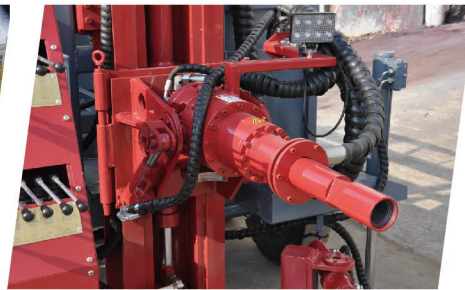
Tilt power head ensures easier and safer loading of Drill Rods
